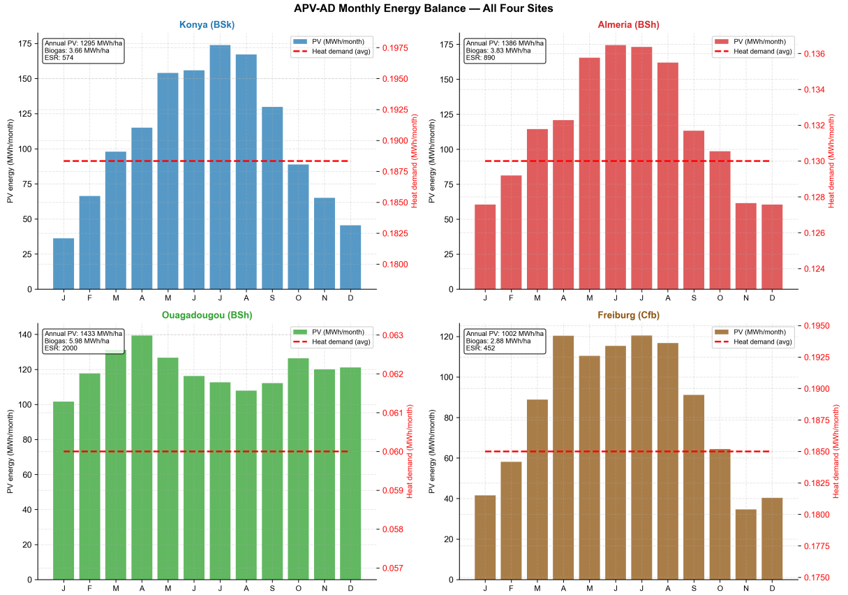
Figure 5: Monthly energy balance for all four sites. Bars: monthly PV generation ( \text{MWh month}^{-1} ). Dashed line: monthly average digester heat demand. The heat demand is nearly constant year-round at all sites because T_{\text{dig,eff}} is clipped to [26, 37]^{\circ}\text{C} (Equation 21), decoupling heat demand from the seasonal PV profile.
