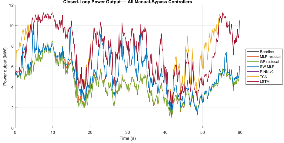
Figure 12: Closed-loop aerodynamic rotor power output, computed directly from C_p(\lambda, \beta) at each simulated state – uncapped (not limited to the 5 MW rated electrical power a real generator and converter would enforce), all seven manual-bypass controllers overlaid ( V = 14 m/s, T = 60 s, seed= 2025).
