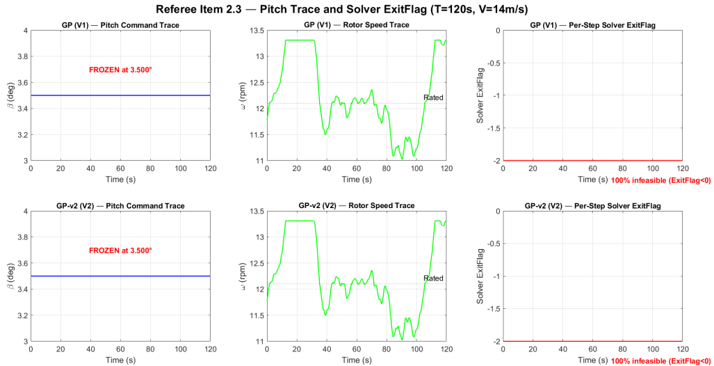
Figure 20: Pitch command trace, rotor speed trace, and per-step solver ExitFlag for GP (V1) and GP-v2 (V2) under the original T = 120 s protocol. The pitch command is frozen at its initial value for the full simulation in both cases ( \text{std} = 0 ), and \text{ExitFlag} < 0 (solver infeasibility) at every one of the 1200 steps tested, confirming the 'zero pitch activity' result is a frozen-actuator artifact rather than genuine regulation.
