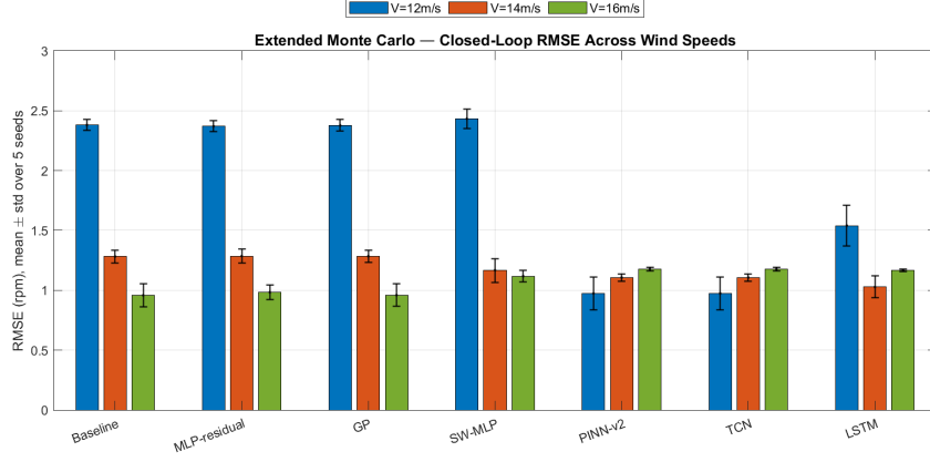
Figure 16: Extended Monte Carlo RMSE across wind speeds, all seven controllers, mean \pm std over 5 seeds.
