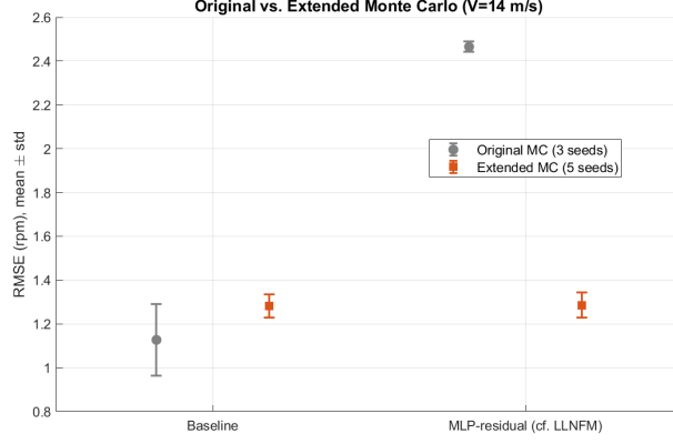
Figure 18: Original (3-seed, single-speed, uncorrected initial condition) versus extended (5-seed, corrected initial condition) Monte Carlo evaluation, Baseline and the MLP-residual surrogate (structurally distinct from, but positioned analogously to, the original LLNFM comparison) at V = 14 m/s.
