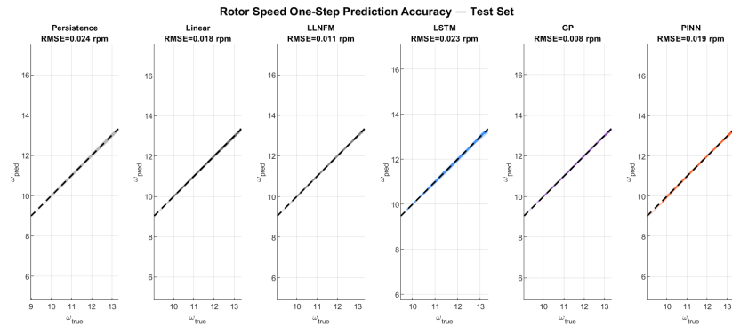
Figure 3: Comparative test-set RMSE across all surrogate models, V1 and V2.
