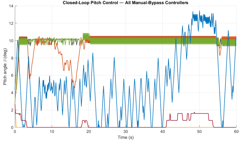
Figure 11: Closed-loop pitch command \beta(t) , all seven manual-bypass controllers overlaid ( V = 14 \text{ m/s} , T = 60 \text{ s} , seed= 2025). PINN-v2's markedly low pitch activity (Table 12) is visible directly as a near-flat trace.
