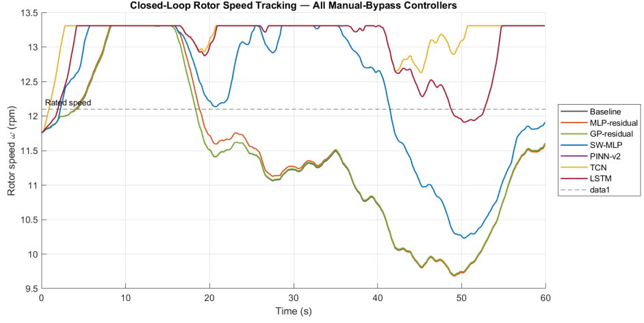
Figure 10: Closed-loop rotor speed tracking, all seven manual-bypass controllers overlaid, V = 14 \text{ m/s} , T = 60 \text{ s} .
