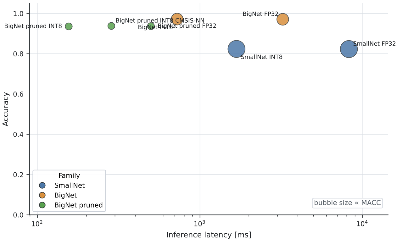
Accuracy vs Inference Latency
