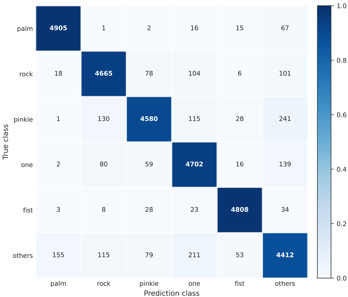
Confusion Matrix — BigNet pruned INT8
