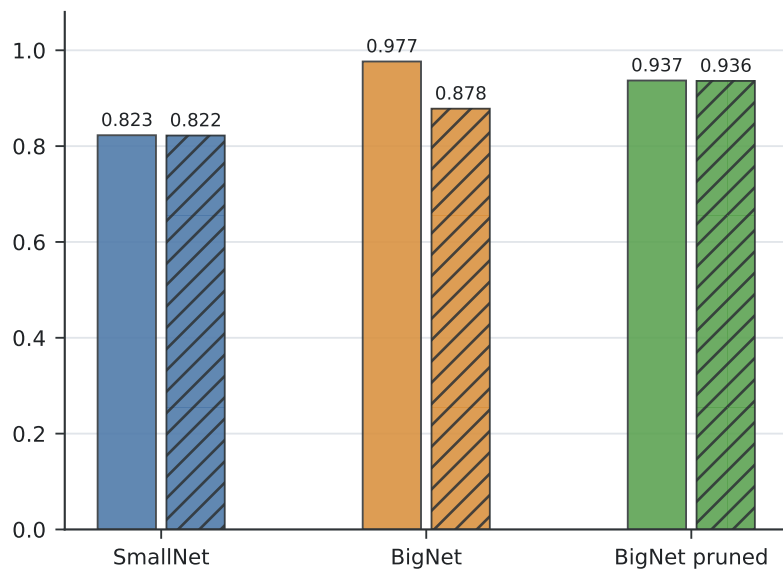
Macro recall
