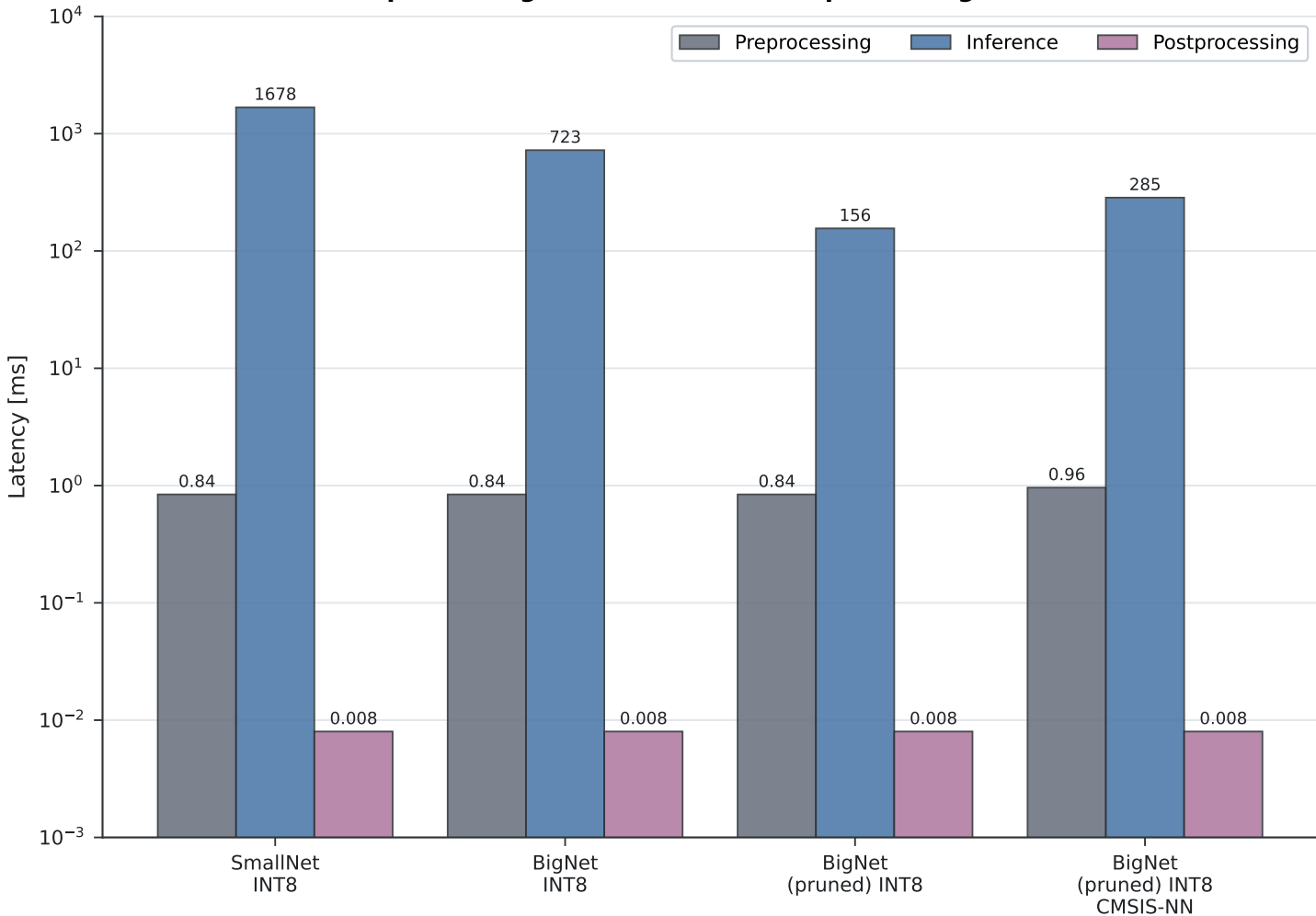
Preprocessing vs Inference vs Postprocessing — INT8
