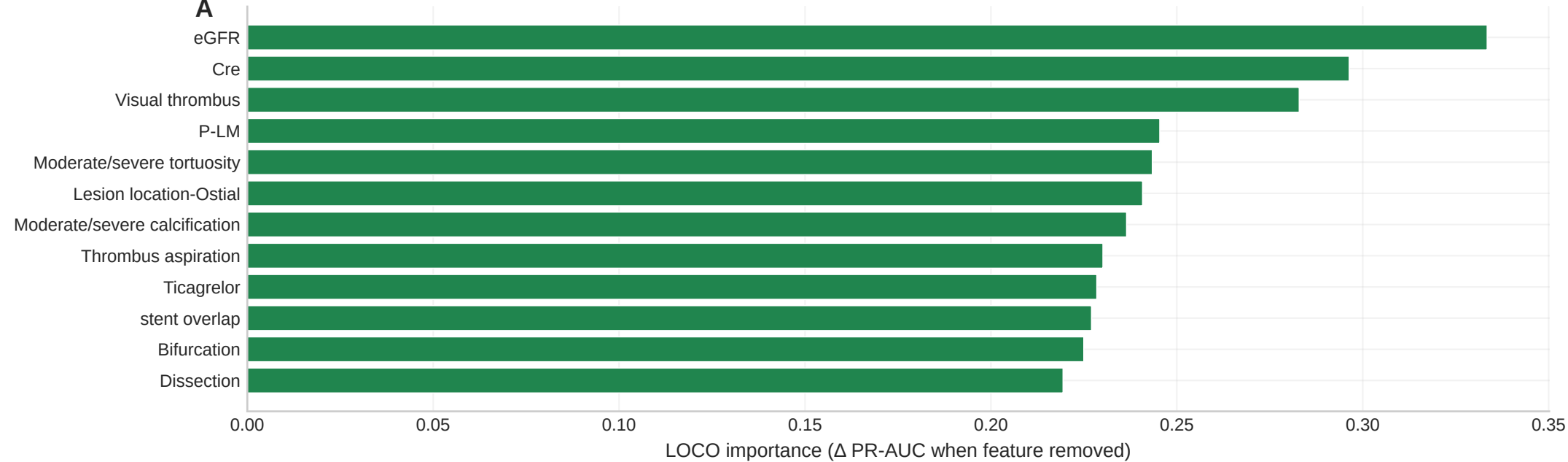
TabPFN leave-one-covariate-out ranking (top 12)
