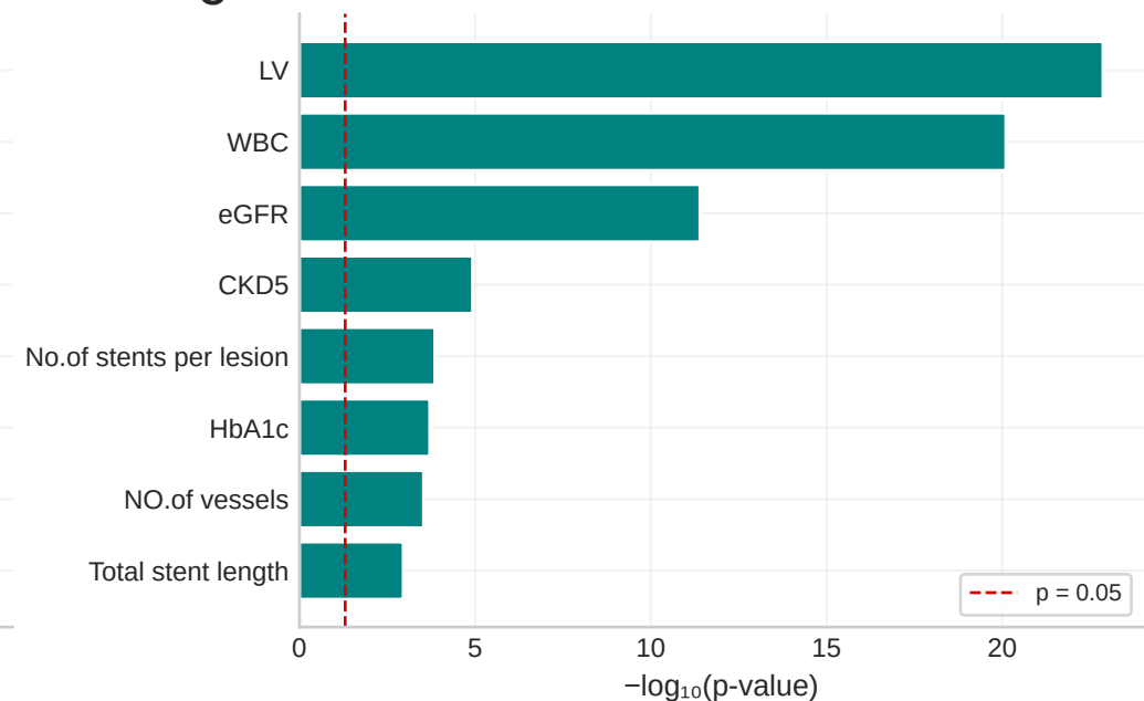
Univariate tests · continuous features
