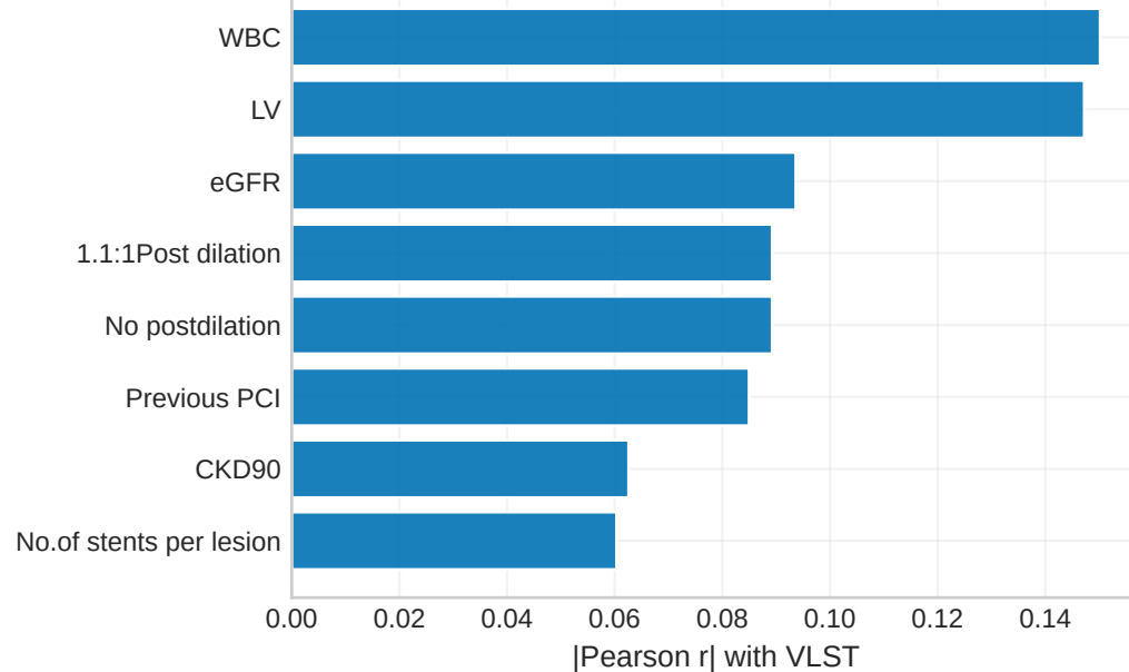
EDA correlation (leakage column excluded)
