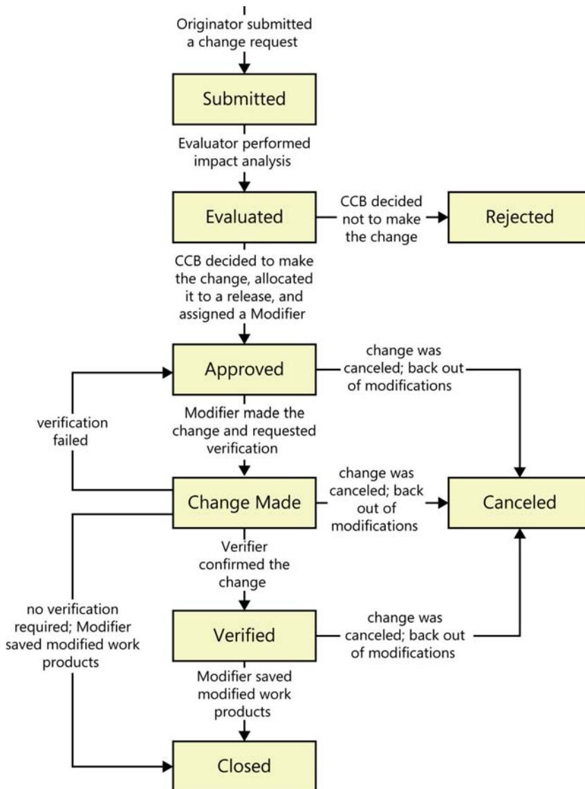
FIGURE 28-2 State-transition diagram for a change request.
