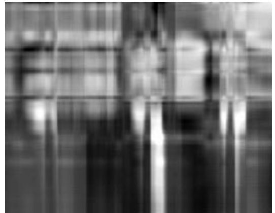
Rank 30 Approximation to Image
