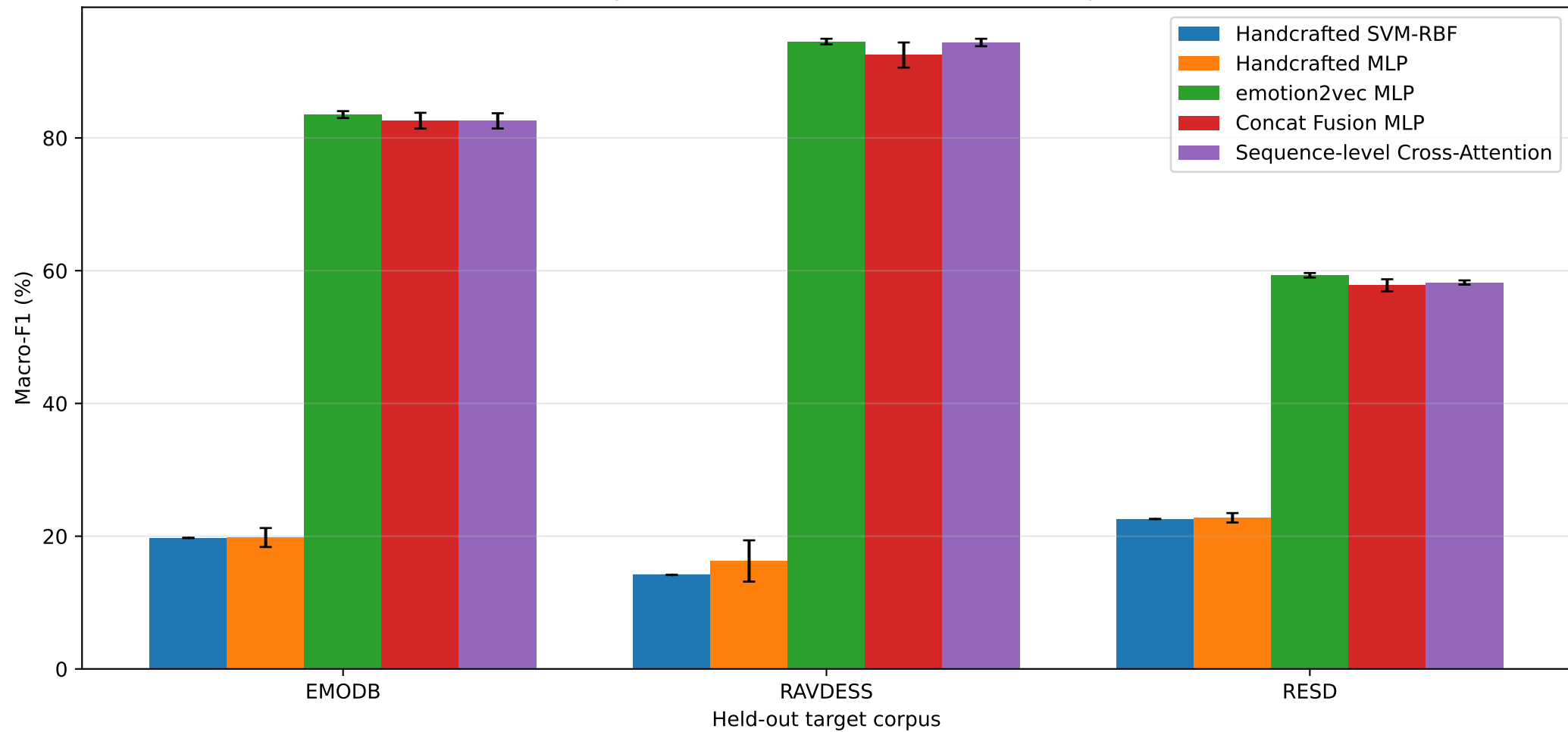
Zero-target LODO Macro-F1 across held-out corpora
