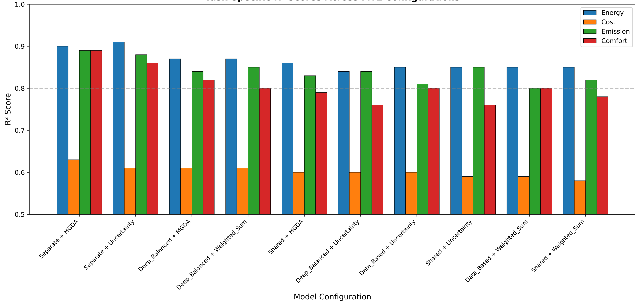
Task-Specific R 2 Scores Across MTL Configurations
