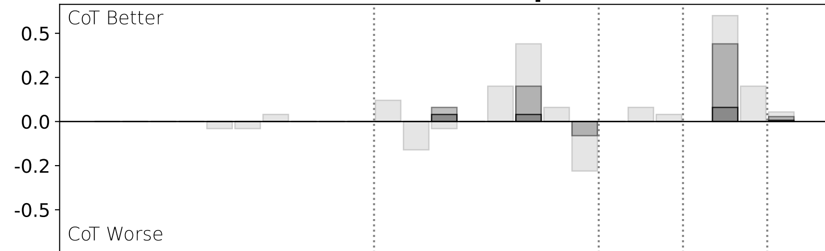
ViPlan-BW: VLM-as-planner
