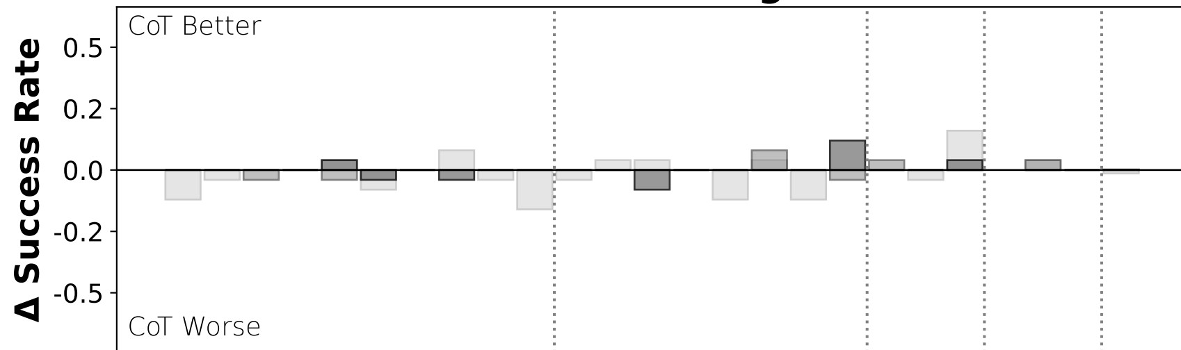
ViPlan-HH: VLM-as-grounder
