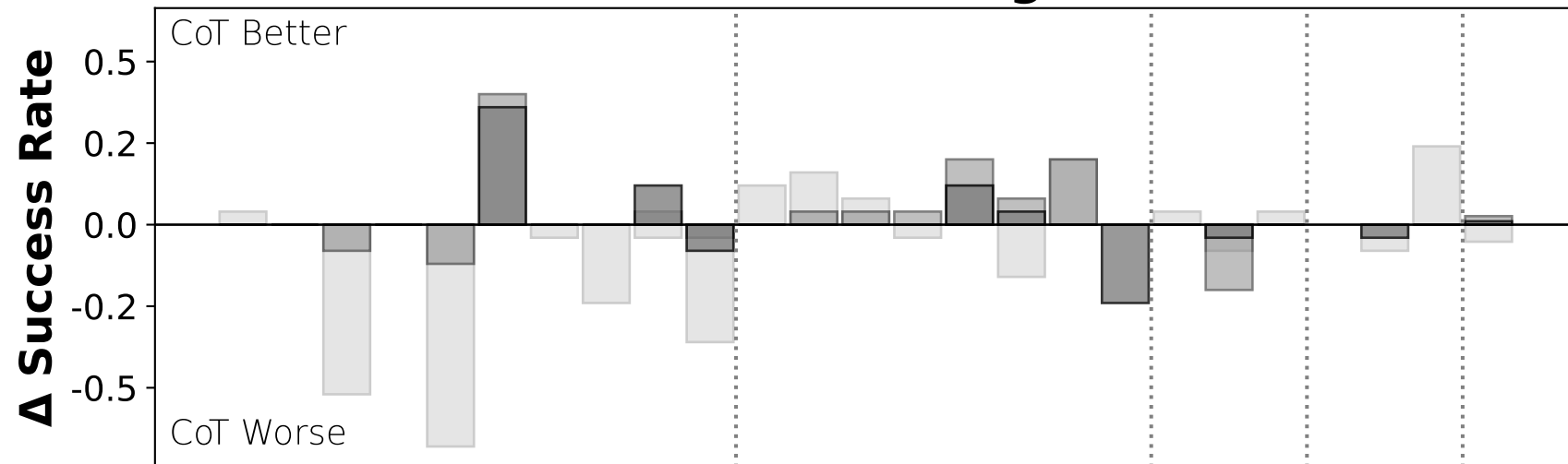
ViPlan-BW: VLM-as-grounder
