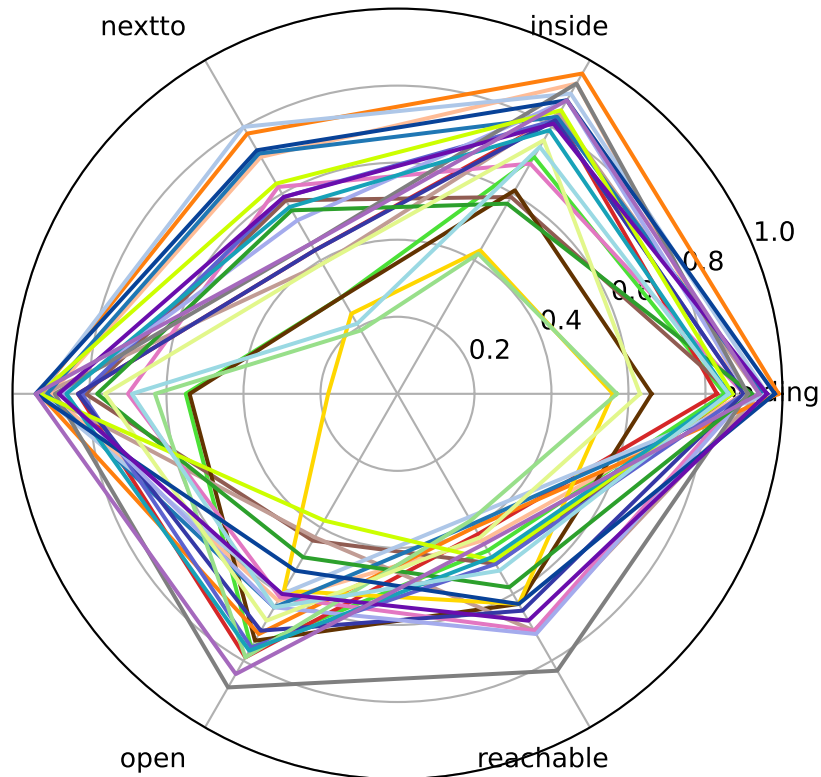
Split: hard
