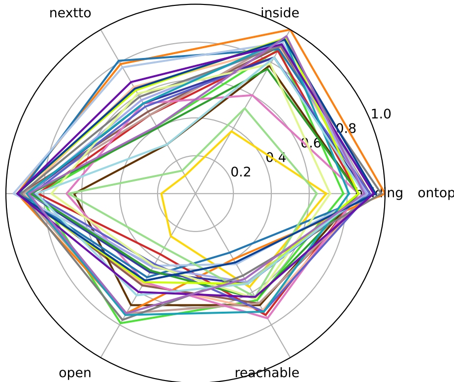
Split: medium
