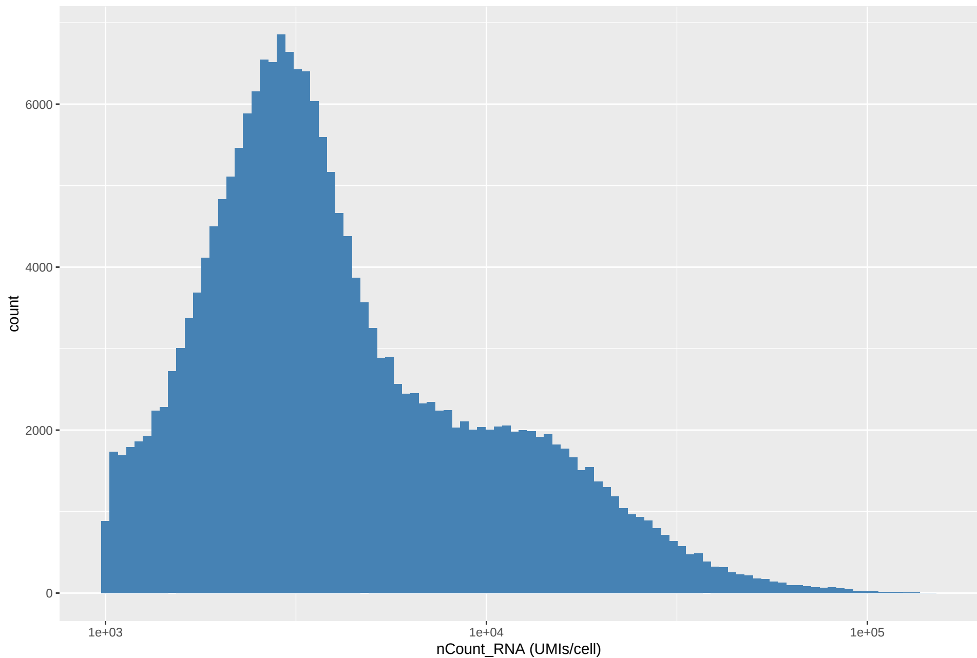
nCount_RNA distribution (log10 x-axis)
