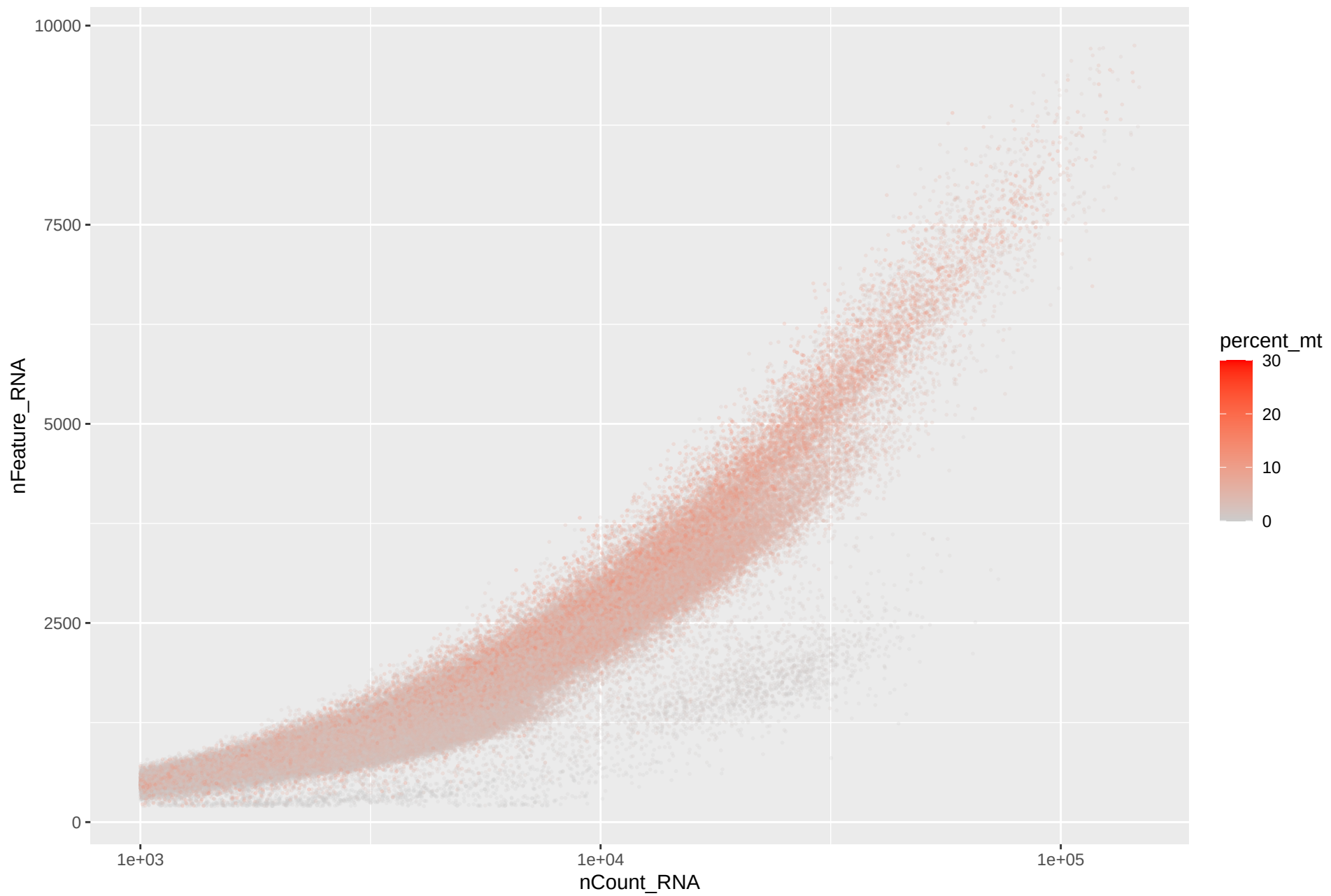
nCount vs nFeature, colored by % mito
