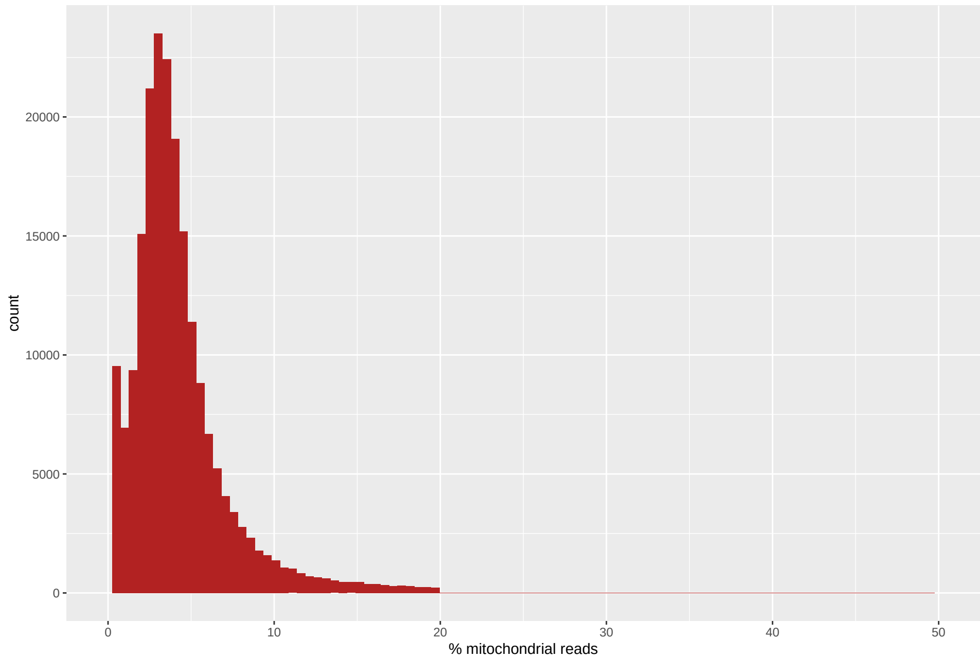
percent_mt distribution (capped at 50% for readability)
