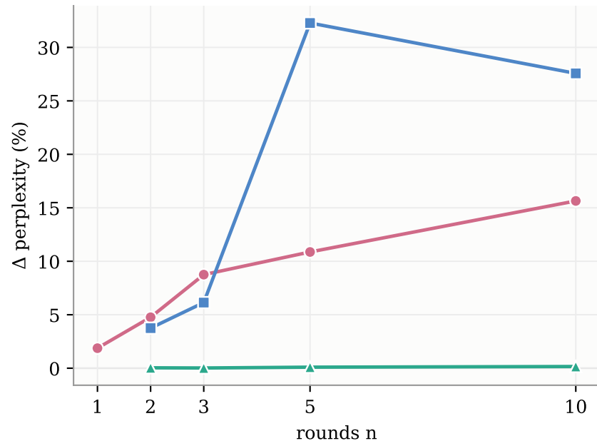
WikiText-2 perplexity
