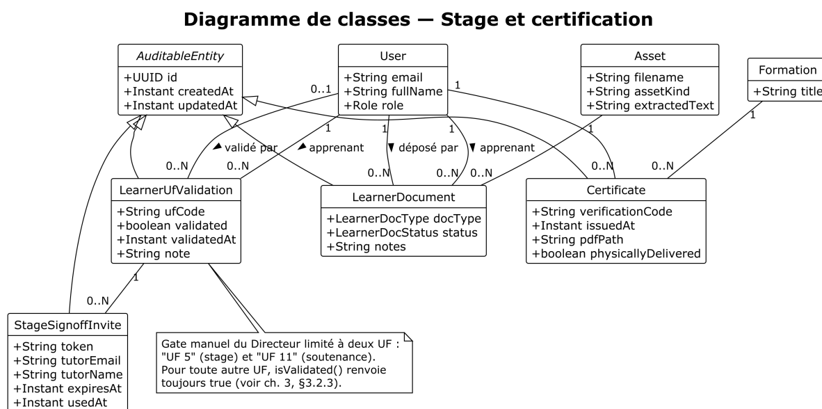
FIGURE 2.5 – Diagramme de classes — stage et certification
