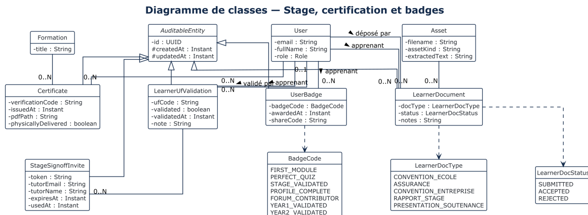
Figure 3.6. Diagramme de classes — stage, certification et badges
