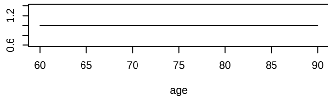
\beta_x^{(1)} VS. x
