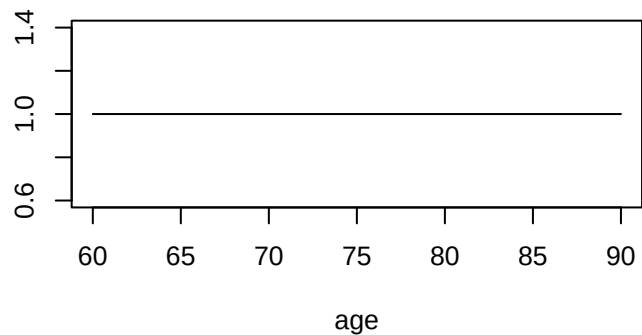
\beta_x^{(1)} vs. x
