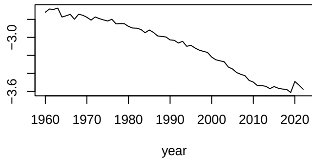
\kappa_t^{(1)} vs. t
