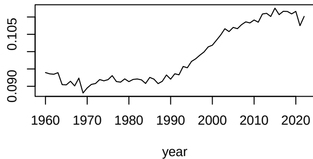
\kappa_t^{(2)} vs. t
