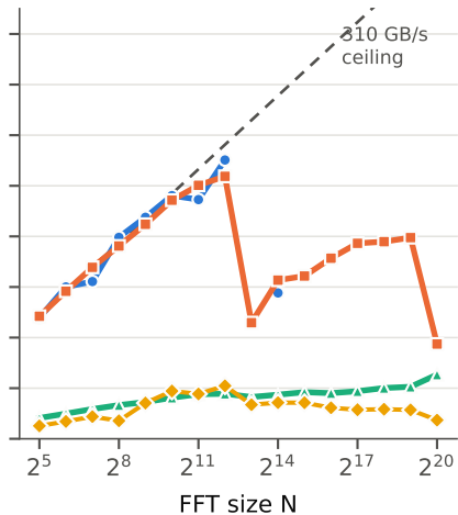
SLC-resident (8 MiB)
