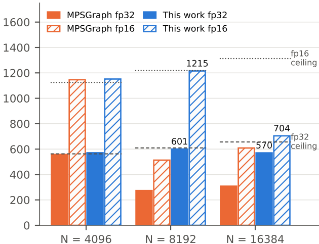
GFLOPS ( 5N \log_2 N )
