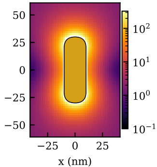
|E|^2/|E_0|^2 , 608 nm
