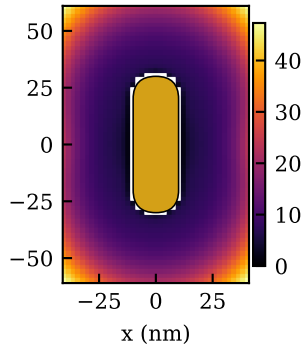
efficiency \langle T \rangle / \langle F_p \rangle (%), 608 nm
