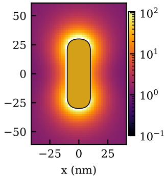
radiative LDOS, 608 nm
