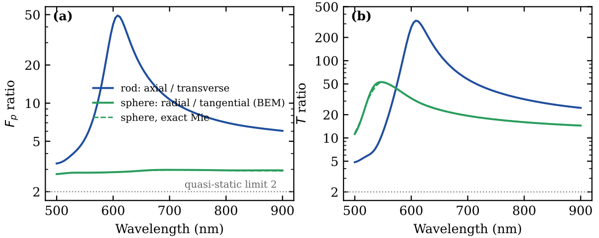
Figure 2: Orientation ratios of (a) F_p and (b) T for the rod (axial/transverse) and the equal-volume sphere (radial/tangential) at a 5 nm gap; dashed: exact Mie solution for the sphere. Dotted: quasi-static flat-surface limit of 2.
