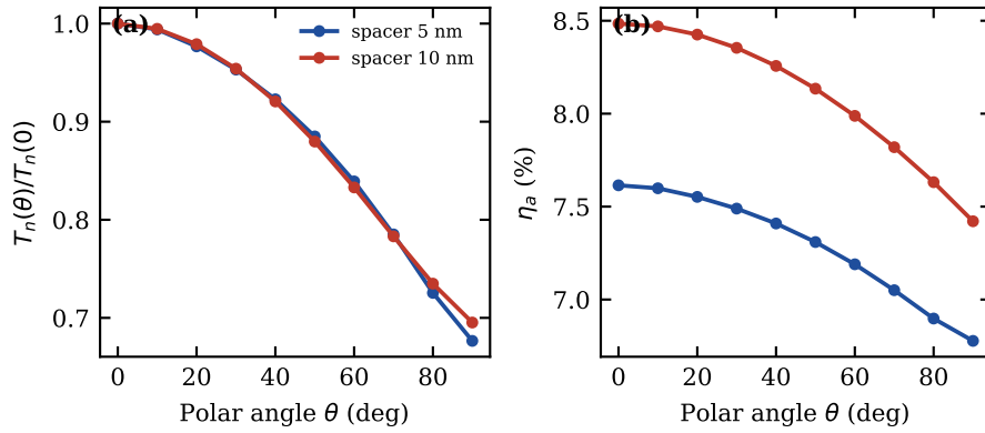
Figure 8: Emitter on a spacer shell of thickness s around the rod tip, at polar angle \theta from the axis, with its dipole normal to the surface: (a) radiative enhancement relative to the on-axis value and (b) antenna efficiency at the radiative peak (610 nm).
