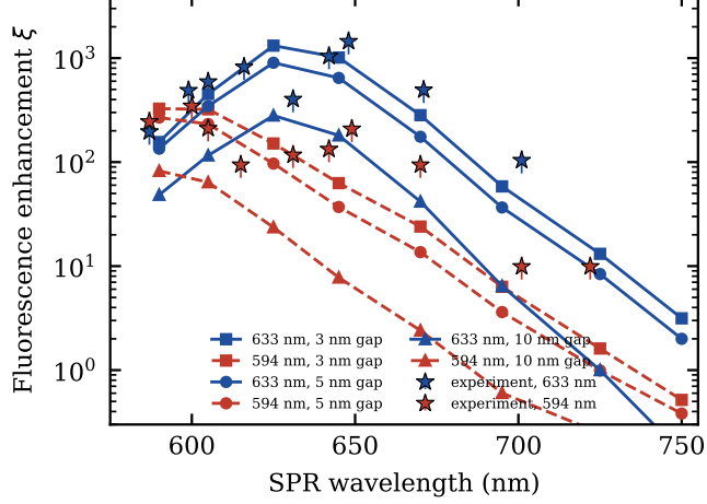
Figure 9: Fluorescence enhancement of crystal violet near gold nanorods of diameter 25 nm in glycerol (BEM, dipole on the axis and parallel to it) versus the computed resonance wavelength, for excitation at 633 and 594 nm and gaps of 3, 5 and 10 nm. Stars: maximum enhancement measured on individual rods by Khatua et al. [29] (digitised from their Fig. 5; bars: \pm 25\% ).
