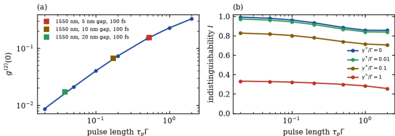
Figure 2. (a) g^{(2)}(0) (b) indistinguishability I (b) as a function of pulse length \tau_p \Gamma for different gap widths (5 nm, 10 nm, 20 nm) at 1550 nm and 100 fs. (b) indistinguishability I as a function of pulse length \tau_p \Gamma for different \gamma^*/\Gamma ratios (0, 0.01, 0.1, 1).
