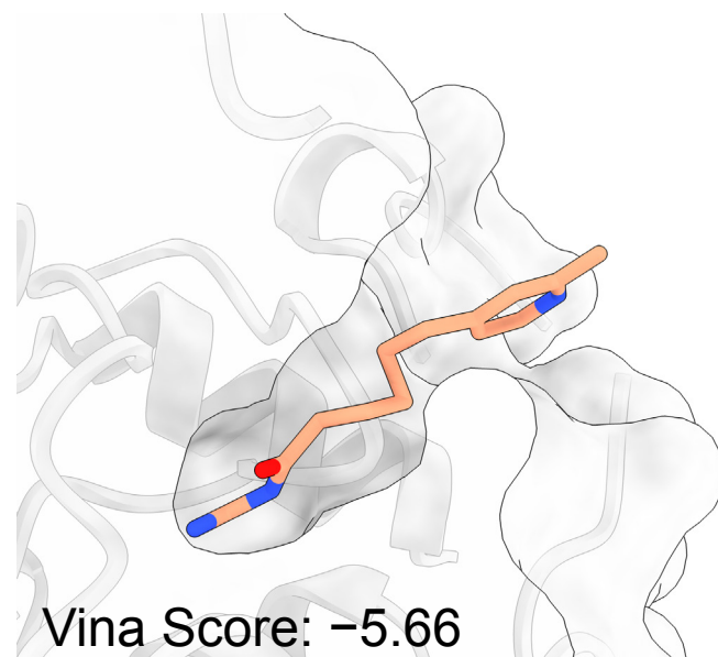
TargetDiff
