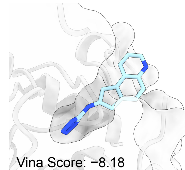
MLIPDiff
