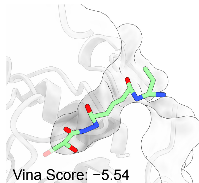
NucleusDiff
