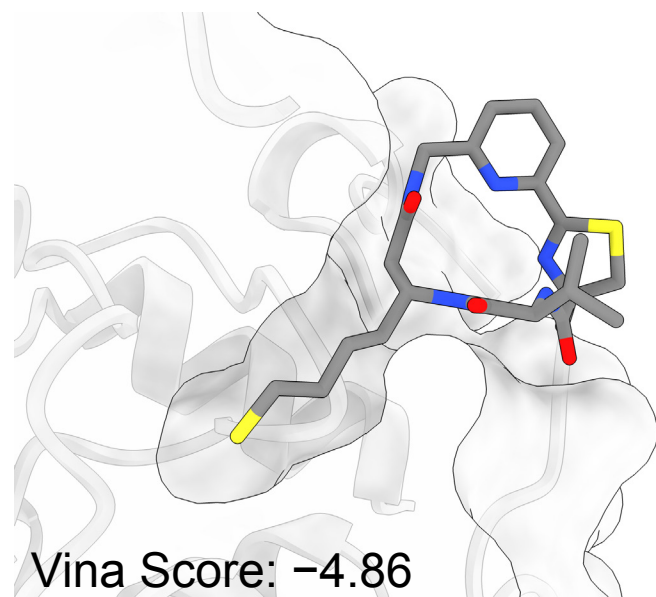
Reference
