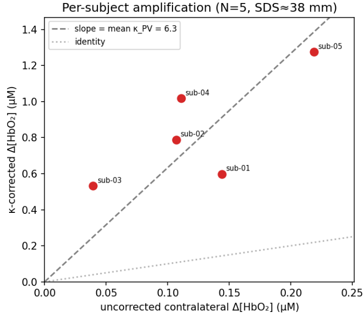
Figure 4: Per-subject amplification for the five BIDS-NIRS-Tapping subjects (contralateral long channels, SDS \approx 38 mm). Each point is one subject’s uncorrected versus \kappa -corrected window-mean \Delta[\text{HbO}_2] ; the dashed line is the mean per-channel \kappa_{PV} \approx 6.3 (only applied amplification) and the dotted line is the identity. Per-subject net scaling varies (4–14 \times ) because the intervening SSR step removes a subject-specific fraction of the raw peak before \kappa_{PV} amplification.
