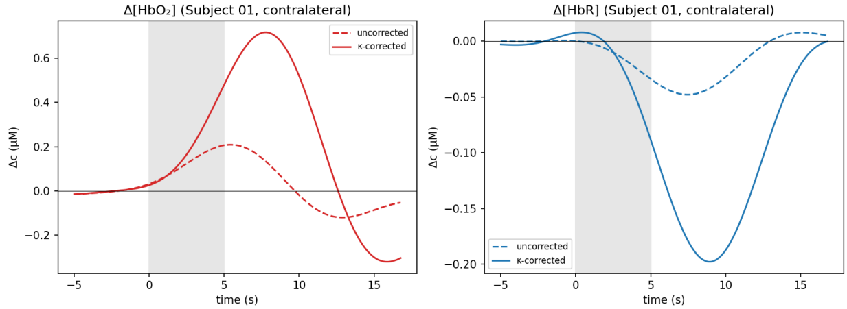
Figure 5: Contralateral block-averaged hemodynamic response (Subject 01, SDS \approx 38 mm), condition-resolved and averaged over the contralateral long channels. Left : \Delta[\text{HbO}_2] . Right : \Delta[\text{HbR}] . Uncorrected (dashed) versus \kappa -corrected (solid, per-channel \kappa_{PV} = 6.28 applied; \kappa_{SSR} diagnostic only). Grey shading indicates the 5 s task period; amplitudes are estimated as the mean over a fixed response window.
