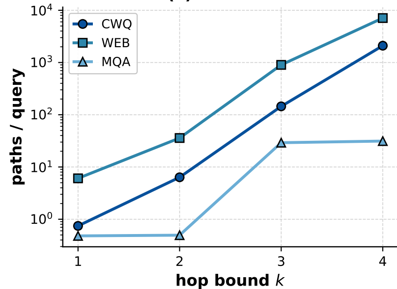
networkx all_simple_paths (no RoG code) reproduces the super-linear blow-up (a) Path count (b) Enumeration latency
