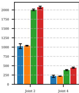
Maximum Transmittable Impedance (N·m/rad)
