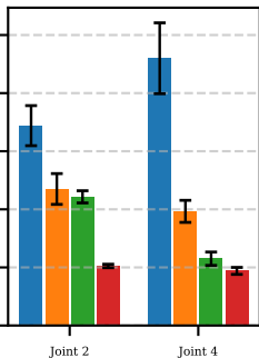
Maximum Transmittable Impedance (N·m/rad)
