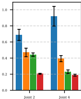
Free Motion Leader's Tracking (NRMSE, %)
