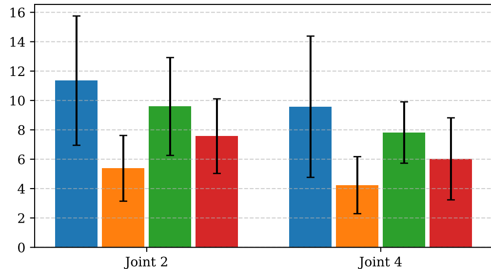
Maximum Transmittable Impedance (N·m/rad)
