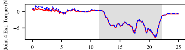
Force Tracking
