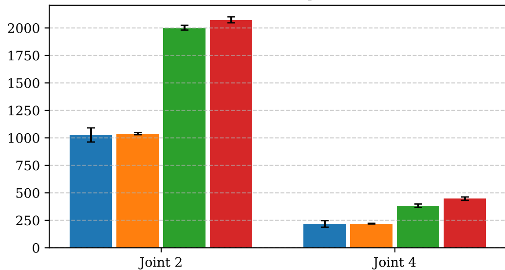
Maximum Transmittable Impedance (N·m/rad)
