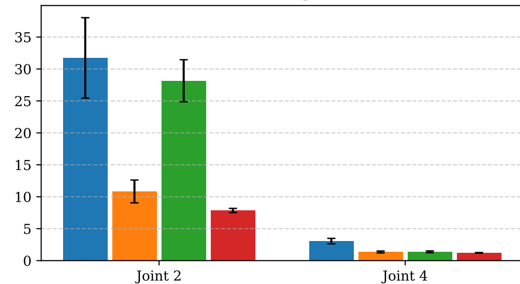
Free Motion Leader's Impedance (N·m/rad)
