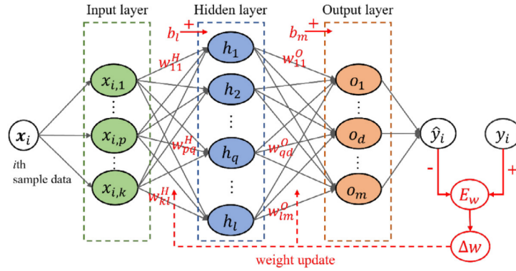
Figure 2.2: The structure of the DNN (Ren & Du, 2023).
