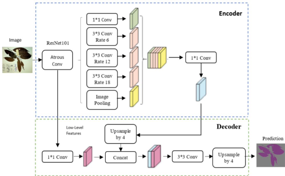
Figure 2.10: DeepLabv3+ architecture (Hussein et al., 2020).
