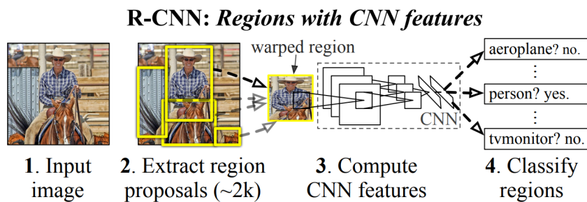
Figure 2.6: Flowchart of R-CNN (Zhao et al., 2019).
