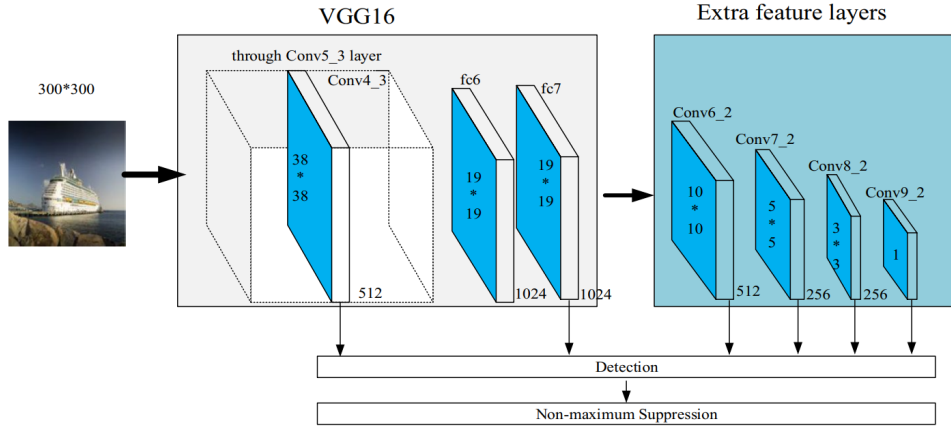
Figure 2.7: Architecture of SSD (A. Li et al., 2021).
