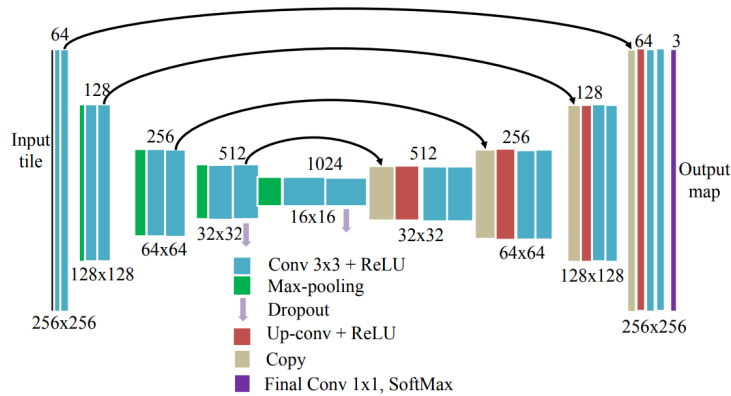
Figure 2.9: U-Net Architecture for Semantic Segmentation (Su et al., 2020).
