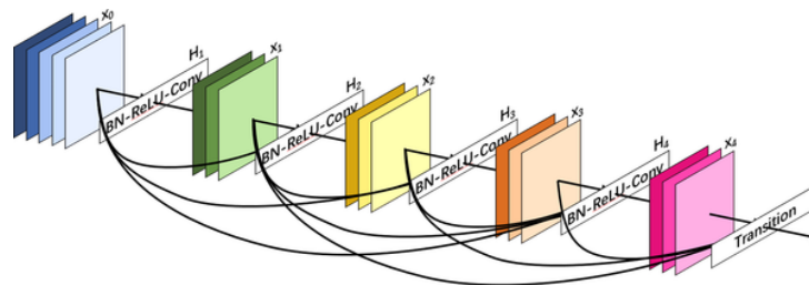
Figure 1.5: The architecture of DenseNet Network (Alzubaidi et al., 2021).
