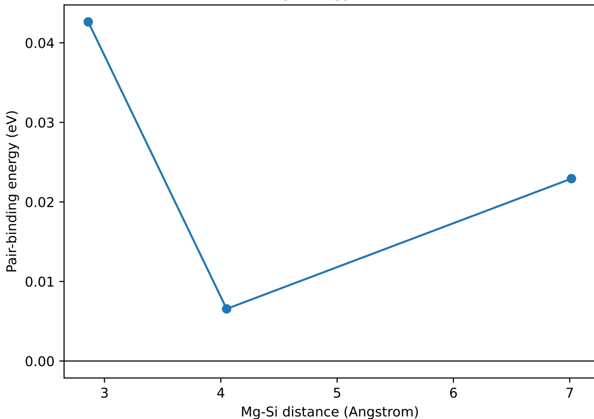
Positive binding energy means attraction
