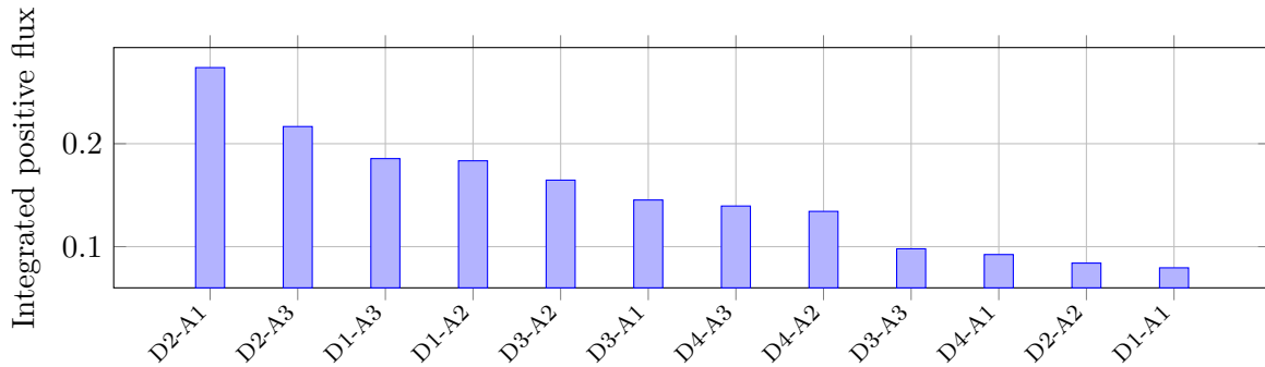
Figure 3: Integrated positive donor-to-acceptor probability fluxes. D_2 \rightarrow A_1 is the most dynamically active pair.
