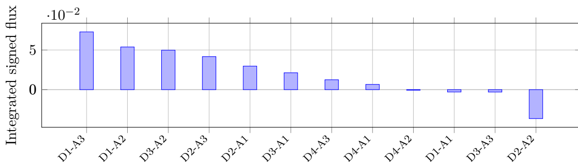
Figure 4: Integrated signed fluxes. Positive bars contribute net donor-to-acceptor population transfer; negative bars indicate net backflow.
