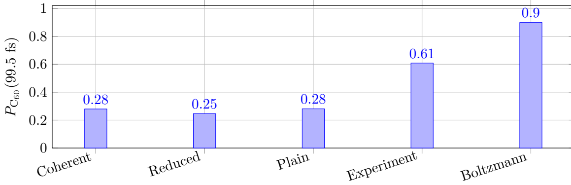
Figure 2: Final C 60 populations at 99.5 fs. The coherent and reduced uncertainties are reported in the text; the FSSH and experiment values are shown without inferred uncertainties.
