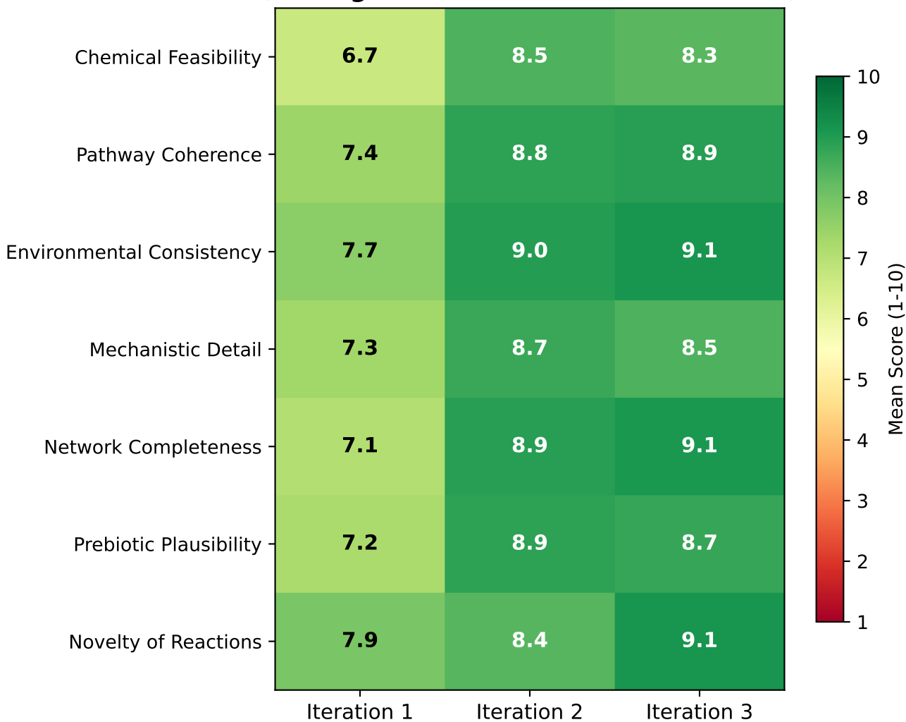
[claude_opus4.6] Mean Criterion Scores by Iteration (averaged across all molecules & runs)
