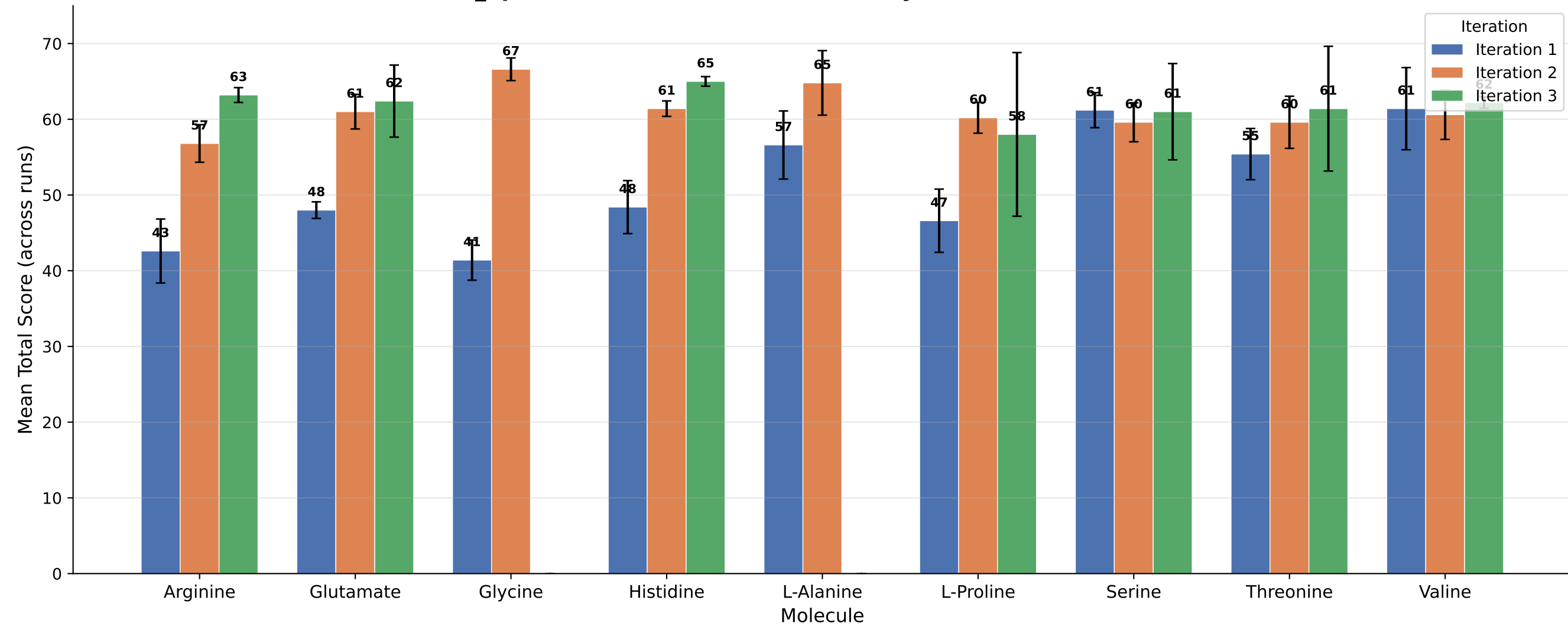
[claude_opus4.6] Iteration Performance by Molecule (Mean \pm Std Dev)
