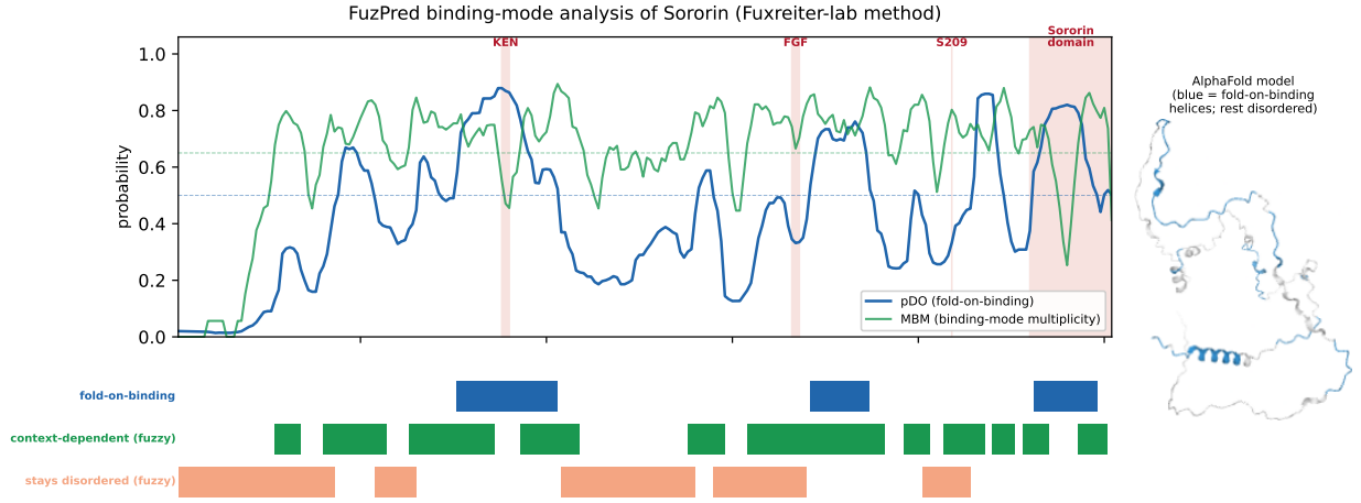
Figure 4: FuzPred binding-mode analysis of Sororin. Left (top), per-residue probability of disorder-to-order (fold-on-binding) binding (pDO, blue) and multiplicity of binding modes (MBM, green); dashed lines mark the 0.5 and 0.65 references and red bands the interaction determinants. Left (bottom), FuzPred region classification in three overlapping tracks (fold-on-binding, context-dependent, and stays-disordered). Right, the AlphaFold model (fold-on-binding helices in blue, the remainder disordered). Most of the protein is context-dependent and multi-mode; only three short segments, including the C-terminal domain, fold on binding.
