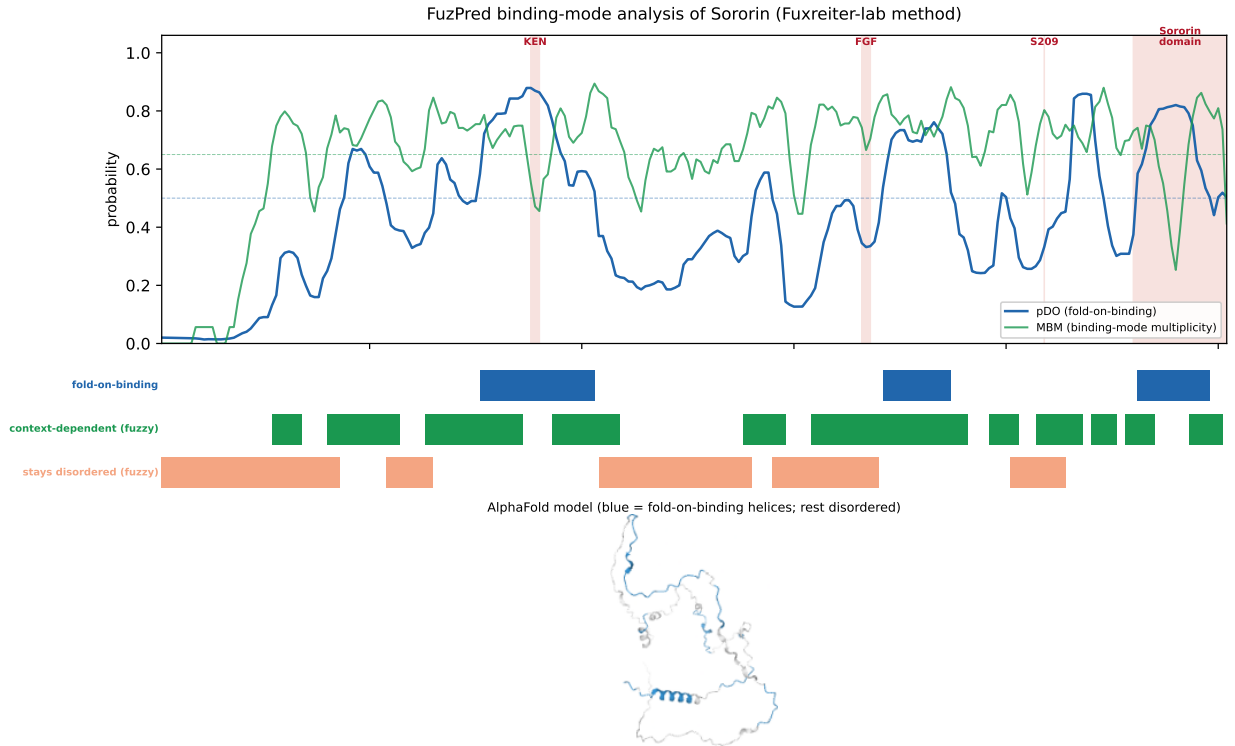
Figure 3: FuzPred binding-mode analysis of Sororin. Top, per-residue probability of disorder-to-order (fold-on-binding) binding (pDO, blue) and multiplicity of binding modes (MBM, green); dashed lines mark the 0.5 and 0.65 references and red bands the interaction determinants. Middle, FuzPred region classification in three overlapping tracks (fold-on-binding, context-dependent, and stays-disordered). Bottom, the AlphaFold model (fold-on-binding helices in blue, the remainder disordered). Most of the protein is context-dependent and multi-mode; only three short segments, including the C-terminal domain, fold on binding.
