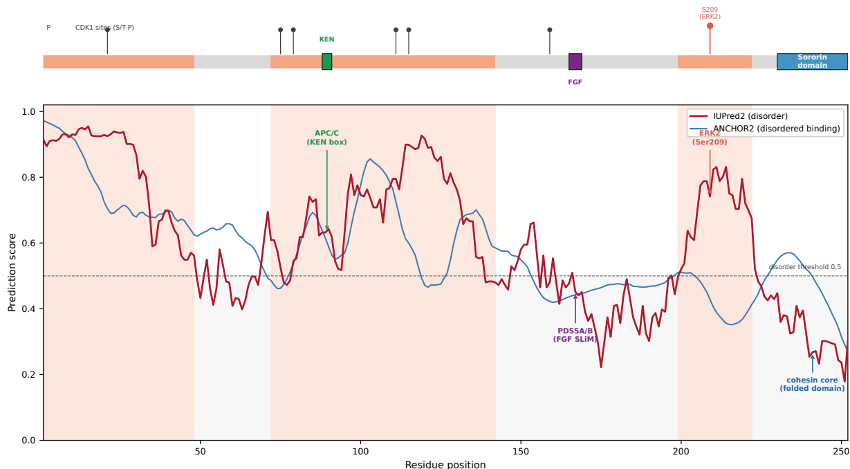
Figure 4: Disorder landscape of Sororin with interaction determinants annotated. Top, domain architecture: three intrinsically disordered regions (orange; UniProt 1–48, 72–142, 199–222), the folded C-terminal Sororin domain (blue), the KEN box and FGF motif, and proline-directed (S/T-P) phospho-sites (lollipop; the ERK2 target Ser209 in red). Bottom, per-residue IUPred2 disorder (red) and ANCHOR2 disordered-binding (blue) scores; the dashed line is the disorder threshold (0.5) and shaded bands mark the annotated IDRs. The APC/C KEN box and the ERK2 site Ser209 fall in disordered regions, the PDS5-binding FGF motif is a short ordered dip embedded in disorder, and the only folded element is the C-terminal Sororin domain.
