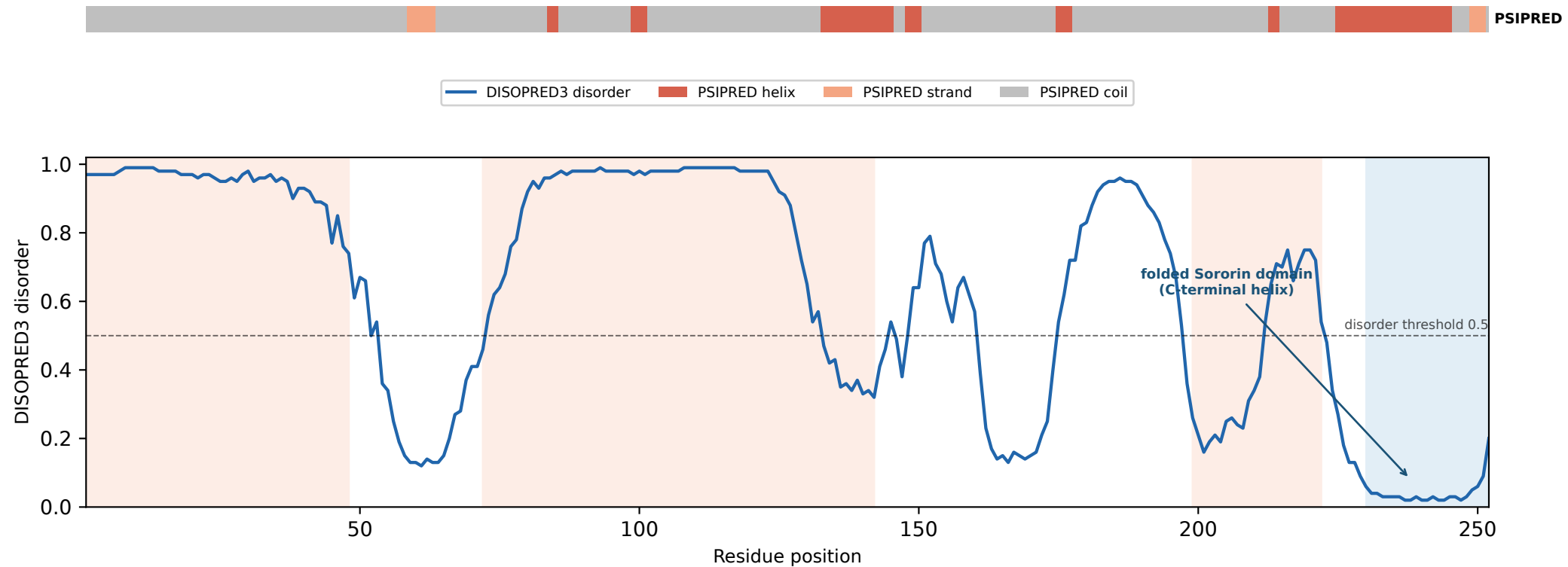
PSIPRED secondary structure over the DISOPRED3 disorder profile of Sororin
