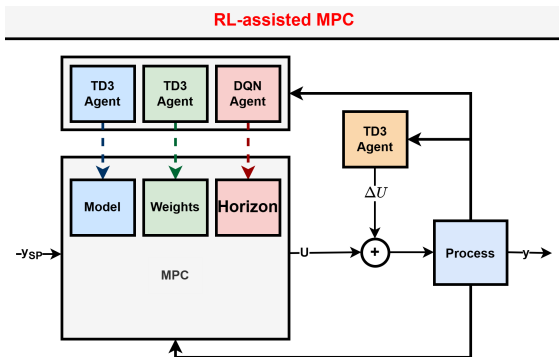
Figure: RL adapts model, weights, horizon, and residual correction around the MPC optimizer instead of replacing it.
