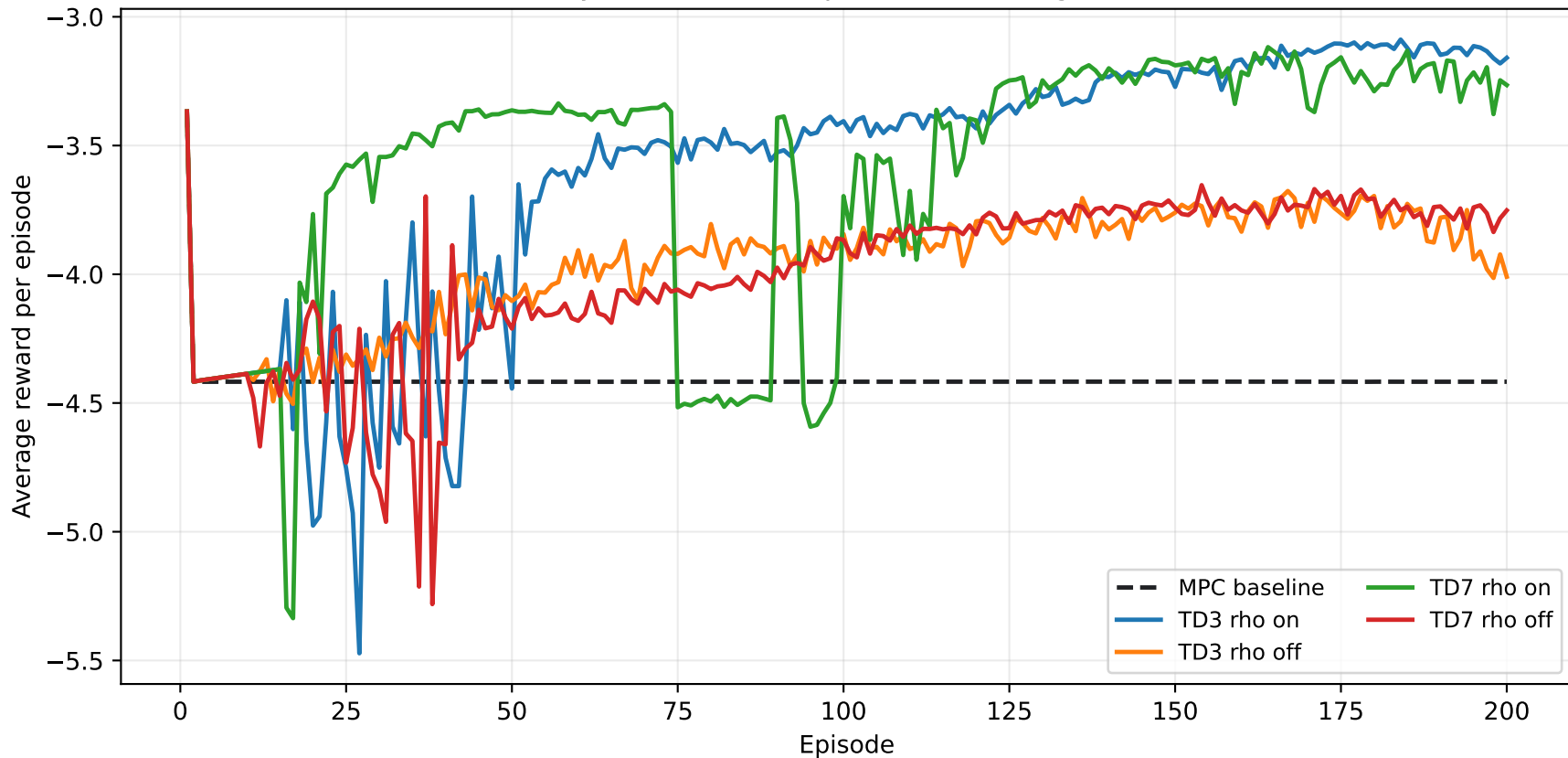
Polymer residual supervisor learning trace
