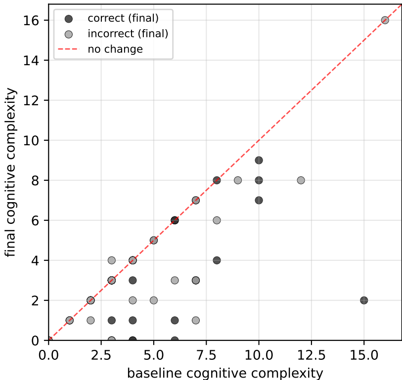
Guarded loop: CogC per task (below diagonal = simplified, safely)
