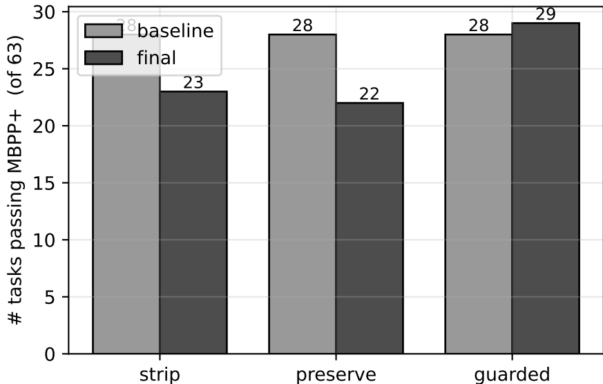
Functional correctness: baseline vs final [H3]
