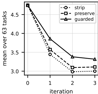
Cognitive complexity
