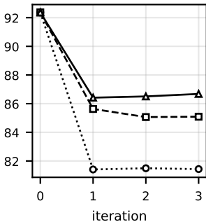
Maintainability Index
