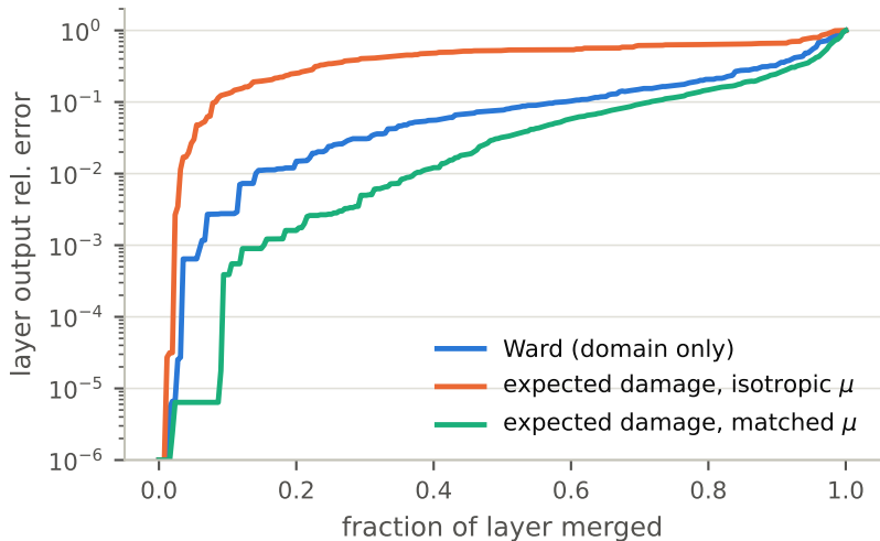
Scoring measures, MNIST layer 0 (3-seed median)
