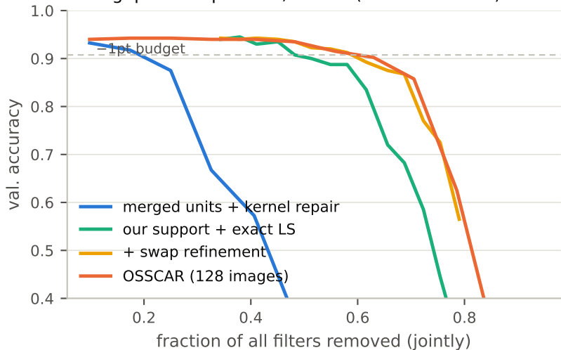
CNN gap decomposition, MNIST (3-seed median)
