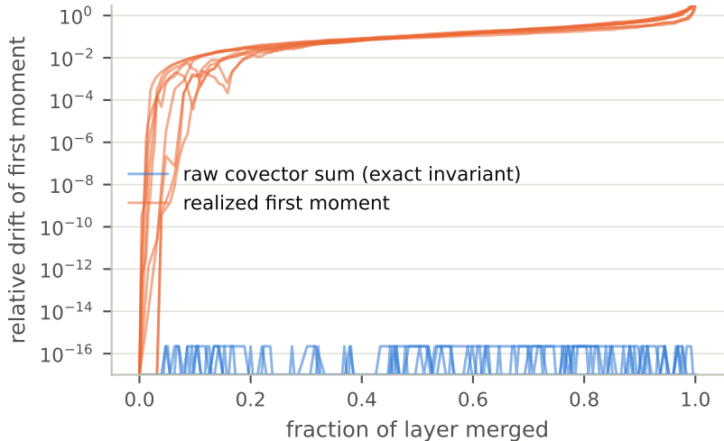
First-moment conservation (all layers, seeds)
