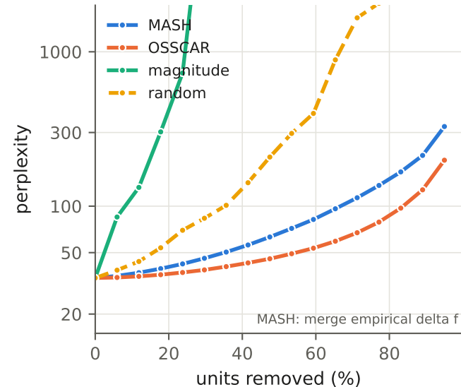
OPT-350m / WikiText-2 (3 seeds)
