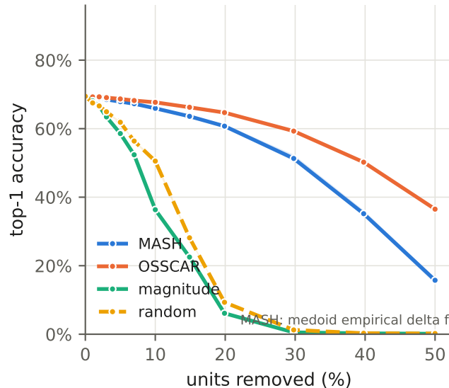
ResNet-18 / ImageNet-1k (3 seeds)
