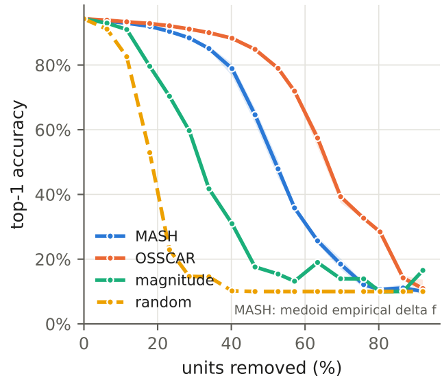
ResNet-56 / CIFAR-10 (3 seeds)
