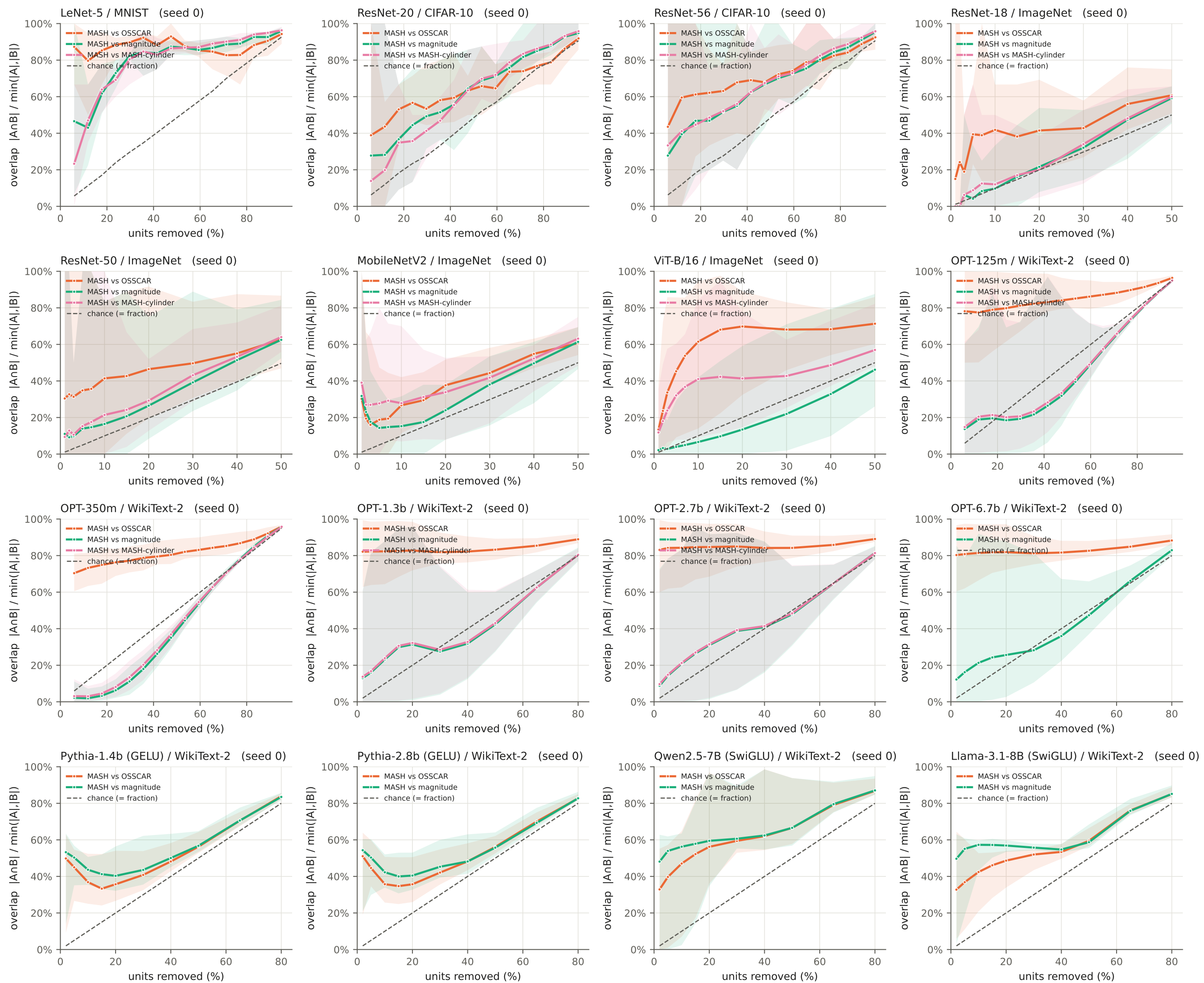
Removed-unit overlap per layer (mean line, min-max band over layers) between MASH delta_f (sampled; merge on FC, medoid under BN) and each other selection. The dashed line is the overlap two independent random sets of that size would have.
