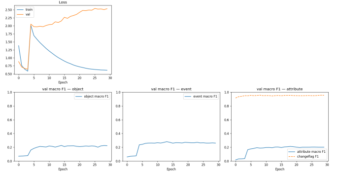
Fig. 2. v3 multitask Phase A training curves. The model converges below the v1 baseline at epoch 15 (best validation avg. macro-F1 = 0.2345) and never improves. The cRT phase (not shown) collapses validation to \approx 0.13 ; the Phase A best checkpoint is used for all inference.
