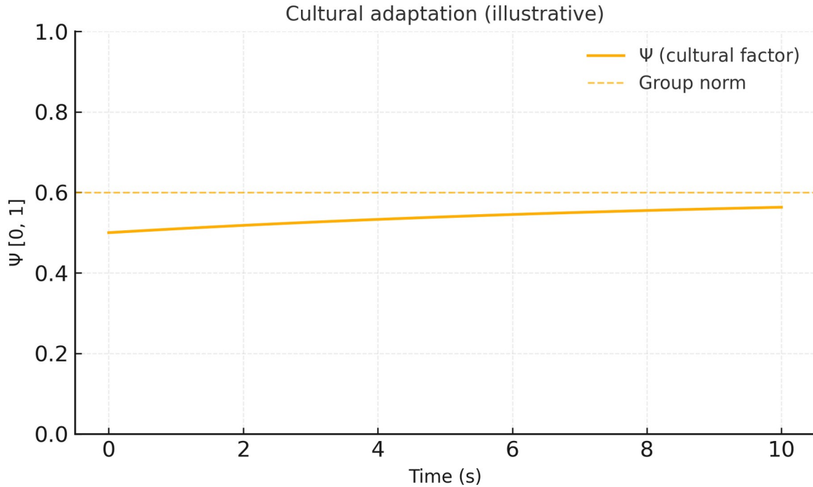
Figure 4. Cultural adaptation in routine dynamics (routine_culture.png). Simulated cultural factor \Psi adapting toward a fixed group norm S_{\text{group}} during the routine-process demonstration. This panel illustrates a simplified first-order cultural adaptation mechanism; parameter values and trajectories are hypothetical and not empirically estimated.
