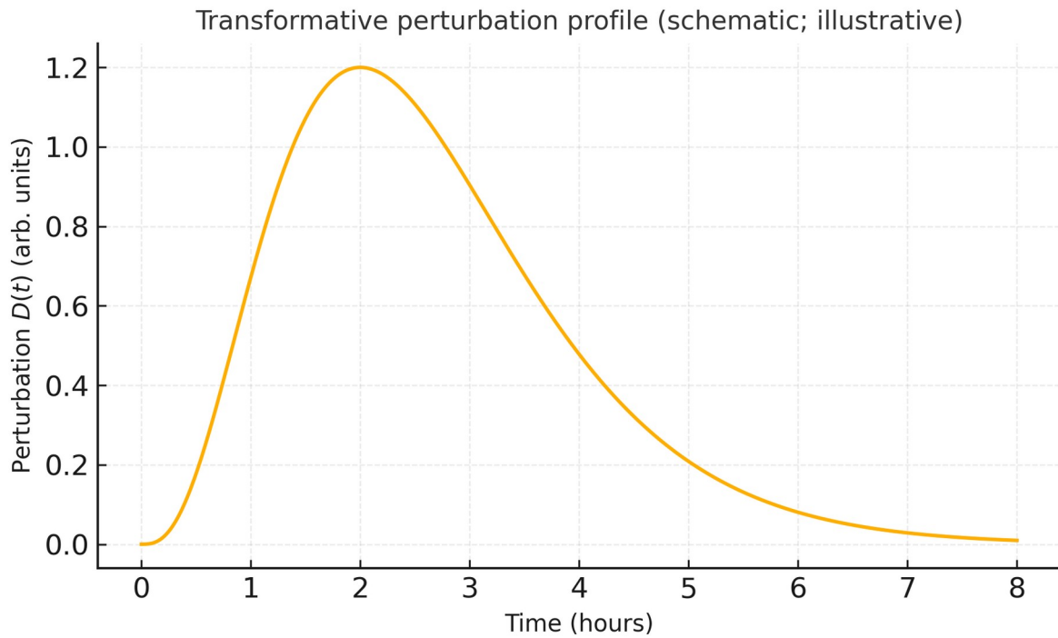
Figure 5. Transformative perturbation profile (transformative_drug_profile.png). Stylized perturbation curve D(t) (gamma-shaped; “psilocybin-like” schematic) used to generate the transformative biphasic demonstration. The profile is a computational convenience rather than a validated pharmacokinetic model. In the exported demonstration, D(t) reaches its maximum (1.20) at t = 2 h and decays toward \sim 0 by 8 h.
