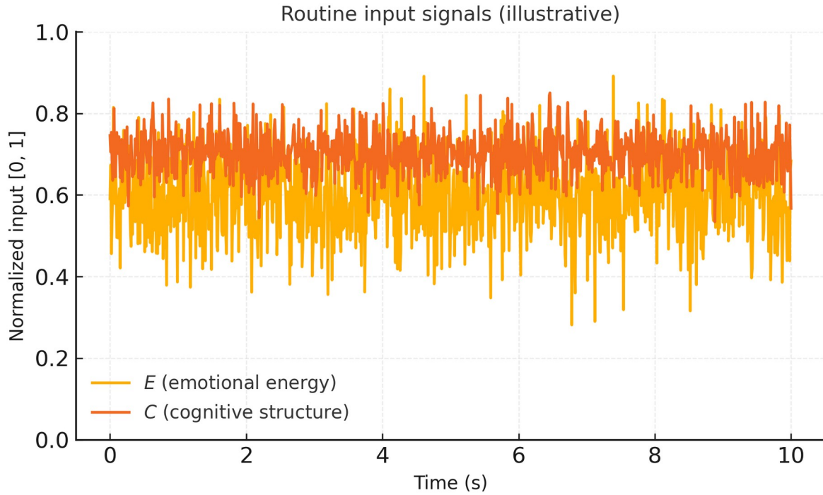
Figure 3. Routine input signals (routine_inputs.png). Stylized input trajectories for emotional energy E and cognitive structure C used to drive the routine-process simulation. Inputs are normalized to [0, 1] and include stochastic variation for illustration; they are not derived from physiological or behavioral recordings.
