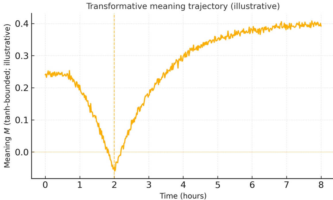
Figure 8. Transformative meaning trajectory (transformative_meaning.png). Simulated meaning signal M_t(t) during the transformative demonstration, shown as a cumulative (time-integrated) quantity computed from the instantaneous simulation-defined meaning signal. This trace is intended to show how meaning could covary with biphasic entropy dynamics; it is not a quantitative model of MEQ30 scores or long-term therapeutic outcomes.
