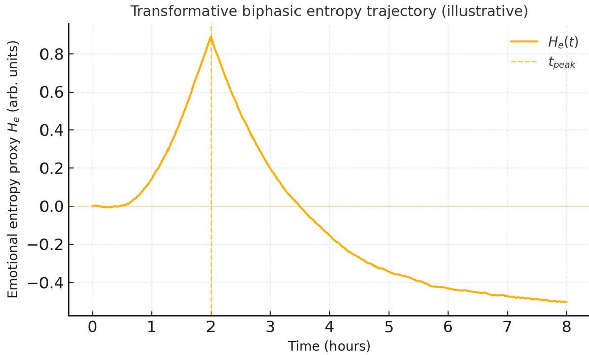
Figure 6. Transformative biphasic entropy trajectory (transformative_entropy.png). Simulated emotional entropy proxy H_e(t) across an 8-hour transformative trajectory exhibiting biphasic dynamics: an elevation phase during onset/peak followed by a post-peak collapse toward a lower setpoint. The dashed line marks the observed peak time ( t_{peak} = 2 h) in the exported demonstration.
