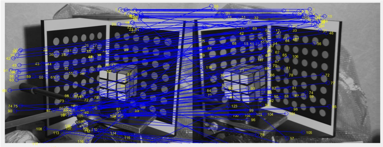
Figure 6: Rubik correspondence points finding algorithm using Sift
