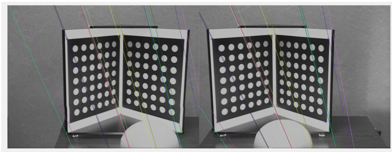
Figure 3: Mire epipolar lines for the algorithm version1
