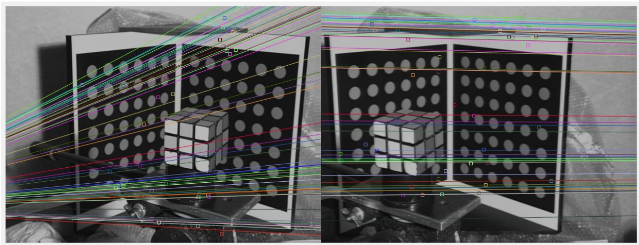
Figure 7: Rubik correspondence points finding algorithm using Sift
