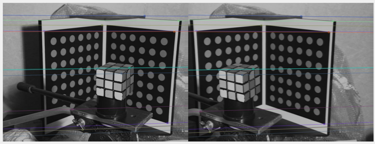
Figure 2: Rubik epipolar lines for the algorithm version2
